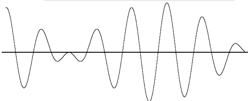
Interference Pattern of Combined Wave
