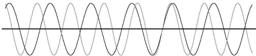
Interference Pattern of Combined Wave
